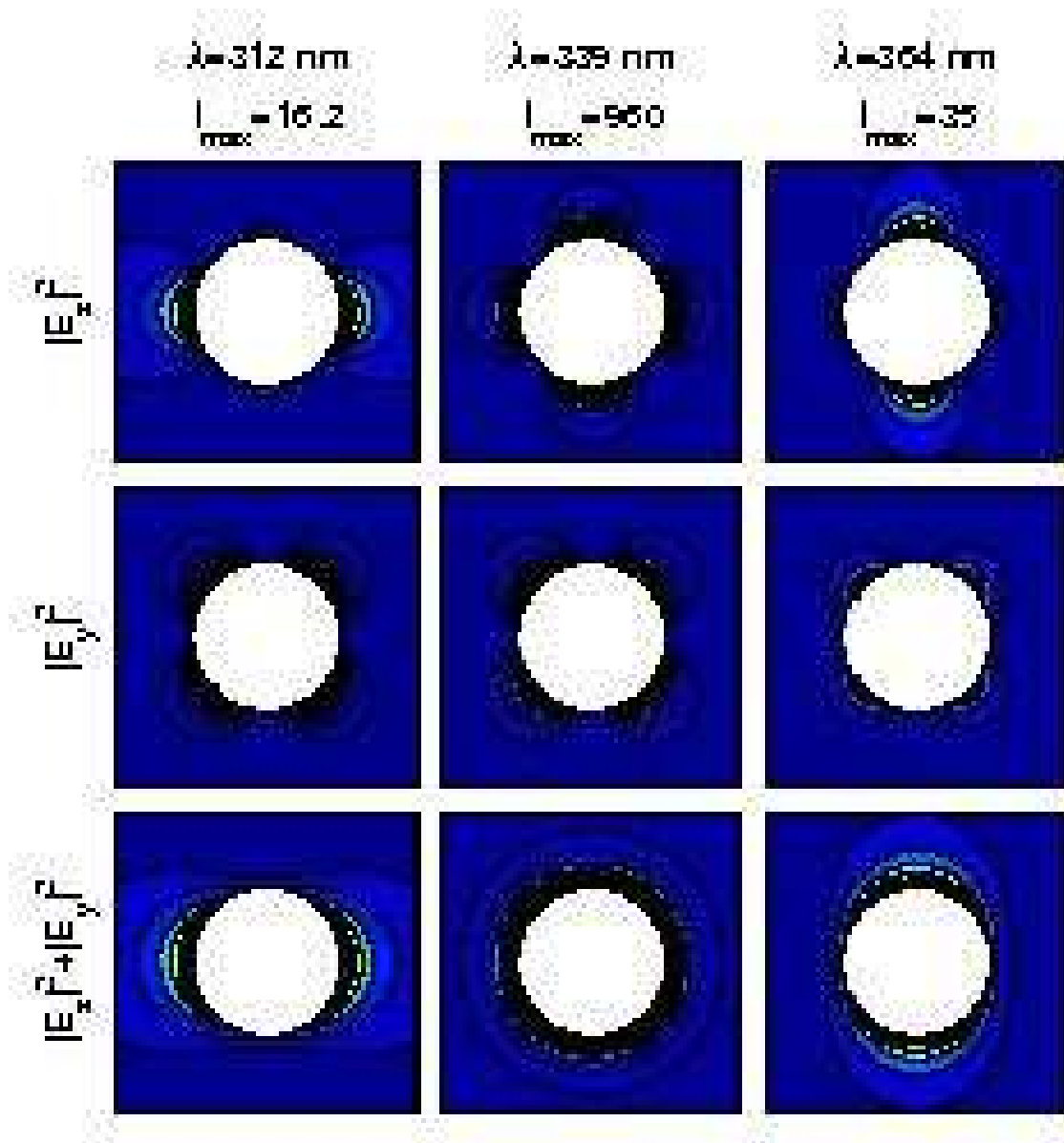
FIG. 2: Intensity patterns in a 2D disk at three different wavelengths (columns) for the field component along z (first row), y (second row), and for the total intensity (third row). The excitation polarization of the external field is along z . For a scatterer with an isotropic Raman tensor, for example, the integrated intensity on the surface of the disk for |E_y|^2 divided by that for |E_z|^2 defines the depolarization ratio \rho . By visual inspection, it is evident that the depolarization ratio will be smaller at 312 and 364 nm than at 339 nm, where the disk has its main resonance. Colors mean different intensities for the different columns; we provide the maximum field intensity for each wavelength at the top of each column. Red (blue) means high (low) intensity in a linear color scale. See the text for further details.
