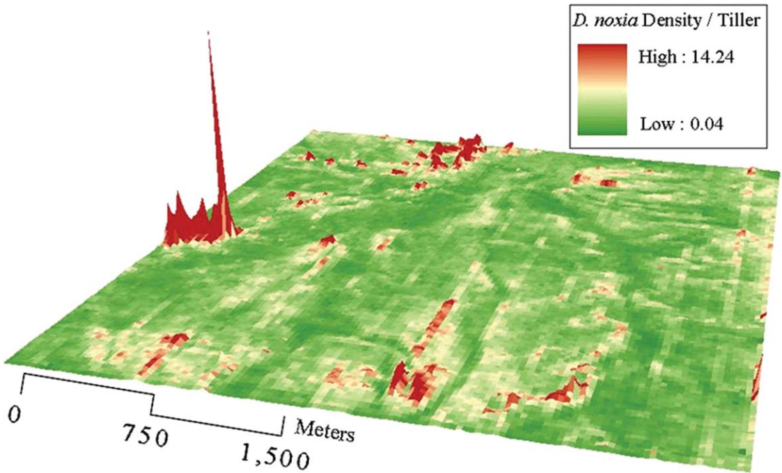
Fig. 1. The modeled D. noxia density trend surface model for the Last Chance Field Site, 25 April 2003 sampling date.
