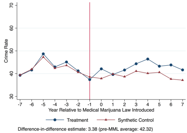
Panel B: Rape
