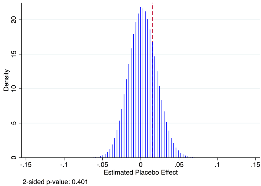
Panel B: Best-fit Placebo Estimates
