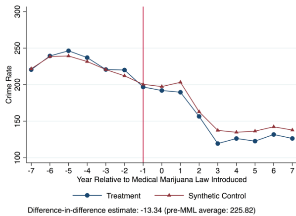
Panel C: Robbery
