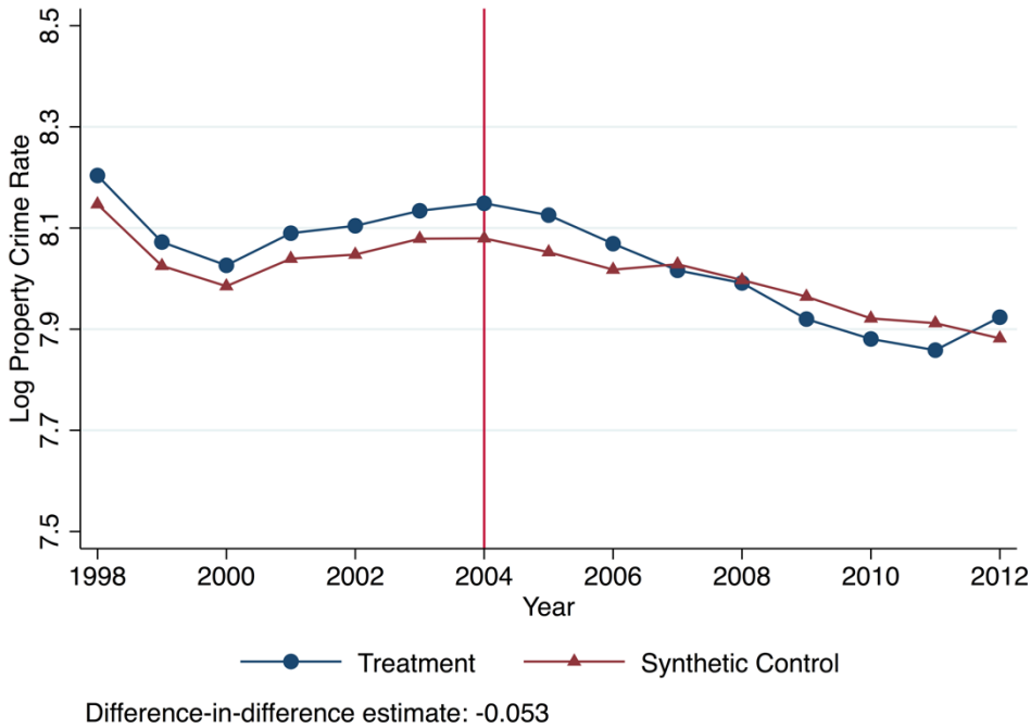
Panel B: Property Crime
