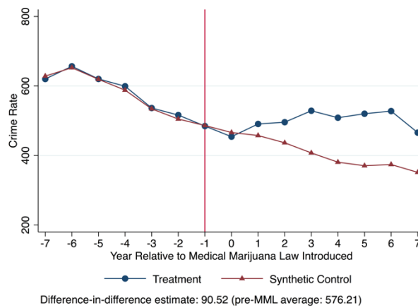
Panel C: Auto Theft
