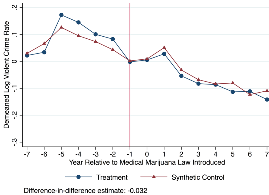
Panel B: Demeaned Log Crime Rates
