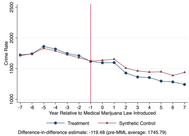
Panel D: Assault
