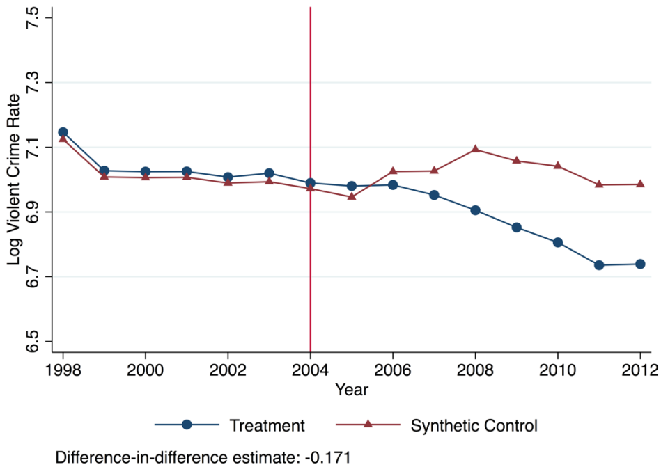
Panel A: Violent Crime
